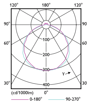
Light Distribution Diagram - ECOFIT E LEDtube 1200mm 14W 765 T8 CT WV
